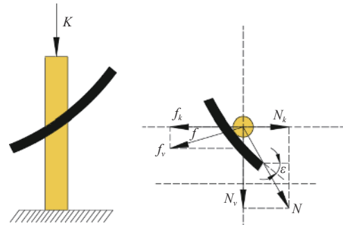
Figure 5 Analysis of straw dynamics at point B
