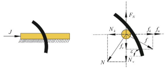
Figure 4 Schematic diagram of wheat straw crushing and mulching
