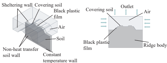
Figure 4 Three-dimensional model of the potato ridge
