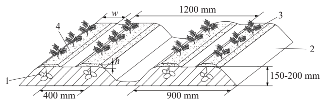
Note: 1. potato; 2. ridge body; 3. seed row; 4. covering soil on the seed row. w is the covering width; h is the covering thickness.
