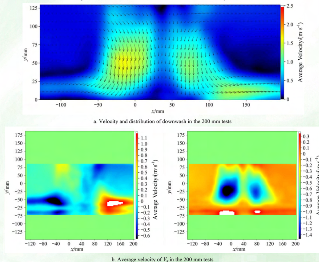
Figure 11 Results of the 200 mm PIV tests of the scaled-down UAV
