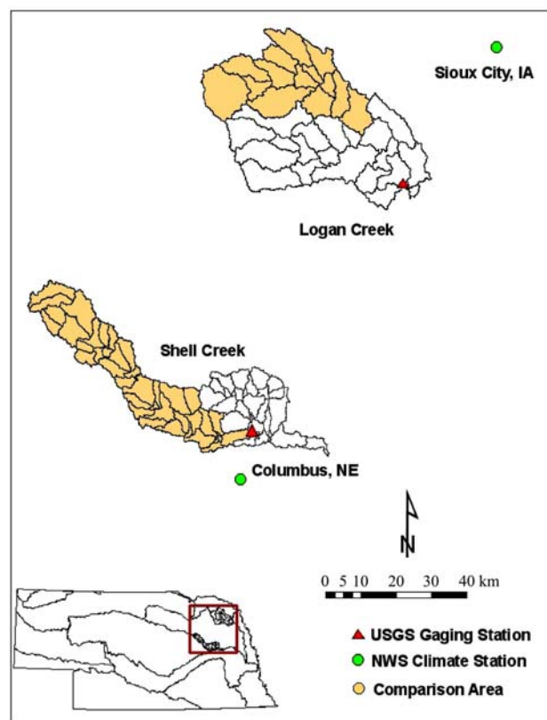
Figure 1 Location of the Columbus, NE and Sioux City, IA climate stations and the Shell and Logan Creek Watersheds
