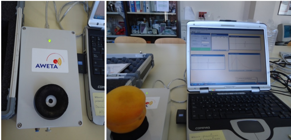
Figure 2 Nondestructive acoustic firmness sensor (AFS)
