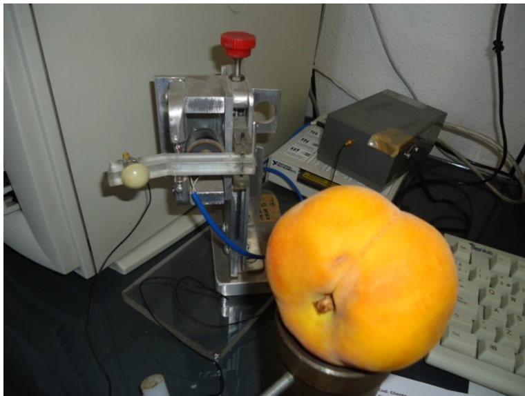
Figure 3 Nondestructive low-mass impact sensor (LPI)
