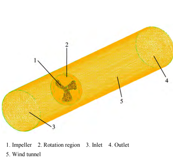
Figure 3 Grid generation of the entity model
