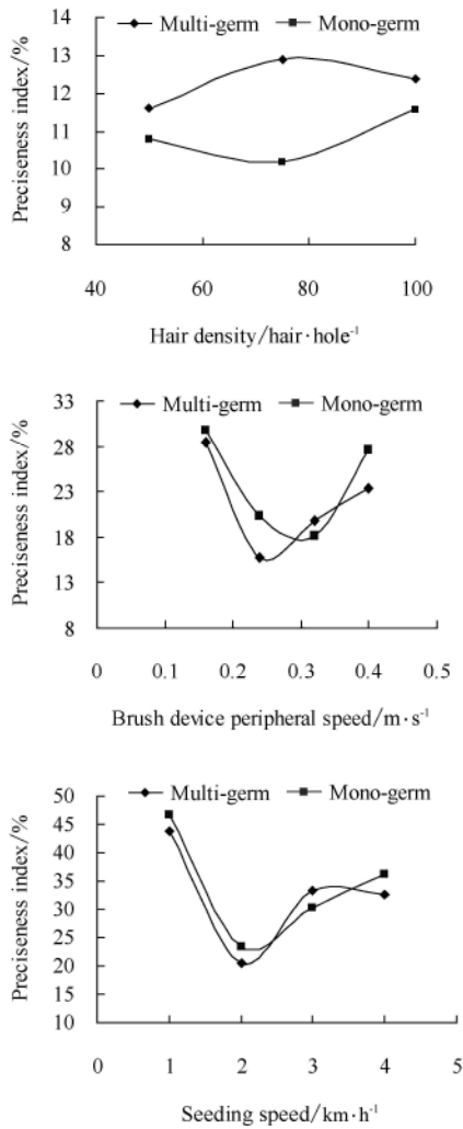
Figure 10 Effect of hair density, peripheral speed and seeding speed on the preciseness indices
