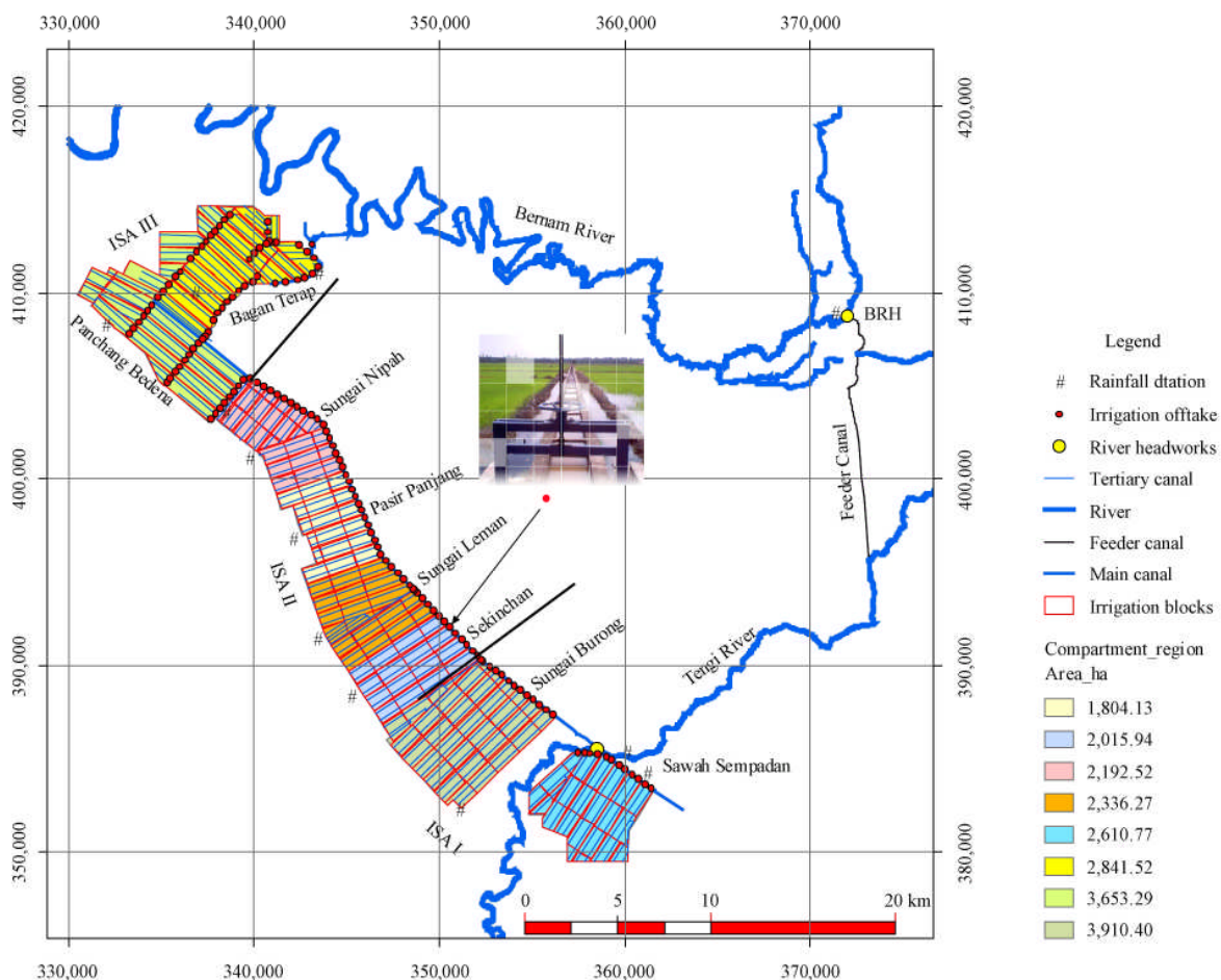
Figure 1 Tanjung Karang rice irrigation scheme
