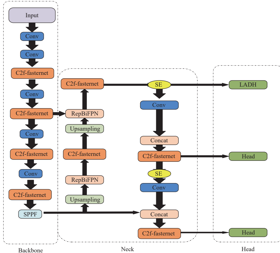
Figure 6 Improved YOLOv8 architecture
