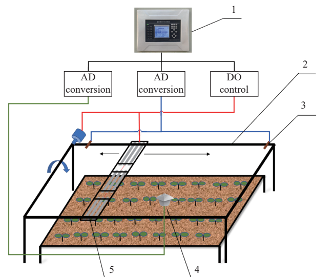
1. Supplemental lighting controller; 2. Gear-rack transmission mechanism; 3. Limit switch; 4. An integrated sensor module; 5. LED supplementary lighting fixtures
