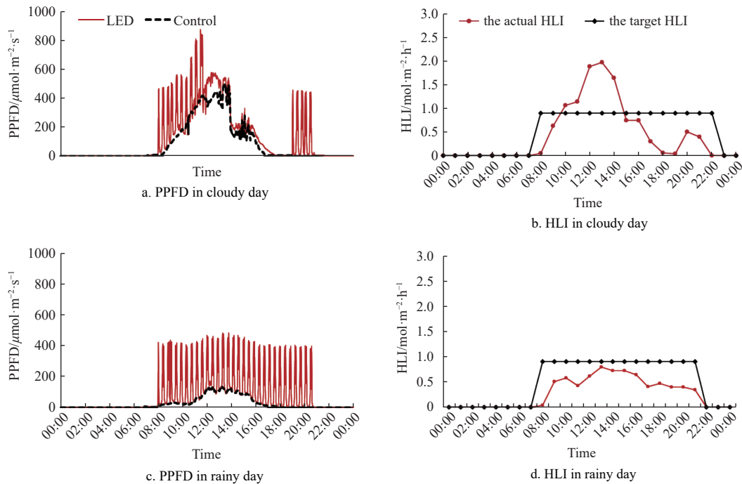
Figure 4 Comparison of PPFD and HLI in the LED supplementary light and control treatments
