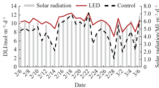
Figure 5 Variations of daily light integral between the supplementary light treatment and control treatments
