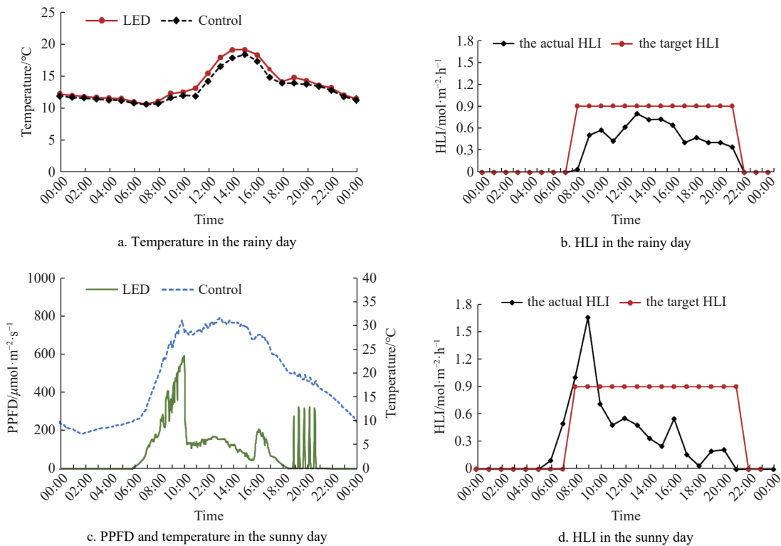
Figure 7 Variations of temperature and HLI in the light-filling treatment under rainy and sunny conditions
