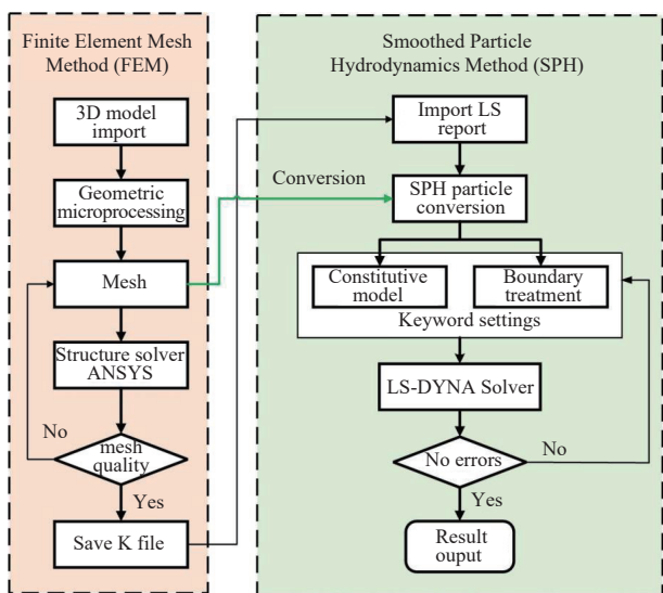
Figure 7 FEM-SPH coupling simulation flow
