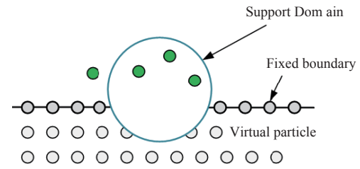
Figure 5 Multi-layer boundary treatment
