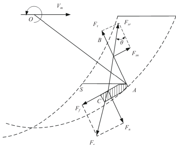
Figure 3 Schematic diagram of resistance to soil cutting by rotary cutter
