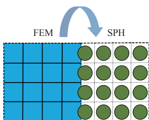
Figure 8 Schematic diagram of node conversion
