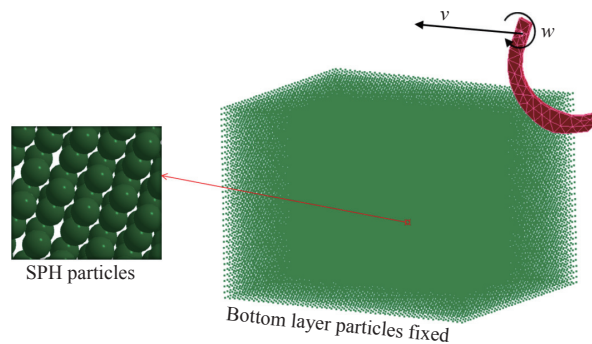
Figure 9 Simulation model of tool-soil interaction
