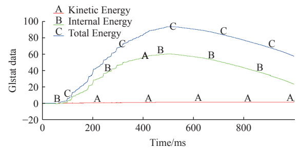
Figure 12 Energy curve of the cutting process
