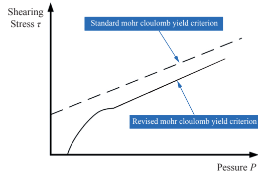
Figure 6 Modified Mohr-Coulomb yielding criterion
