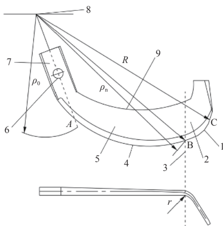
1. Tangent cutting edge 2. Front cutting part 3. Bend line 4. Side cutting edge 5. Side cutting part 6. Mounting hole 7. Tool shank 8. Rotation center of cutter roll 9. Back edge curve
