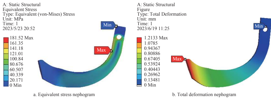
Figure 15 FEM simulation results
