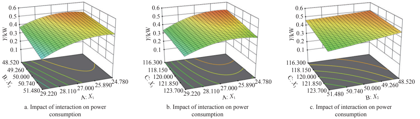
Figure 14 Interaction response surface of various factors
