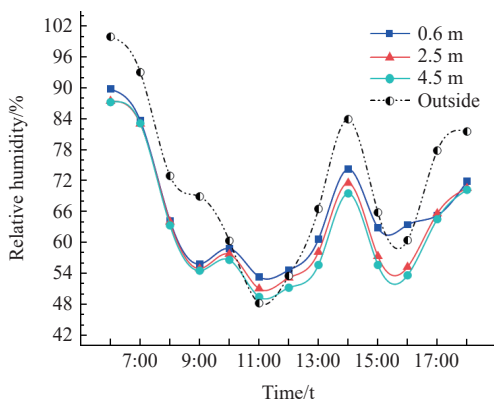
Figure 6 Average relative humidity and outdoor humidity changes at different monitoring heights in the greenhouse at each time
