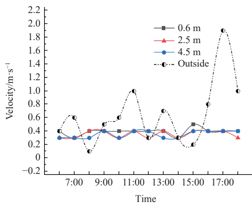
Figure 9 Average speed change at each time in the greenhouse
