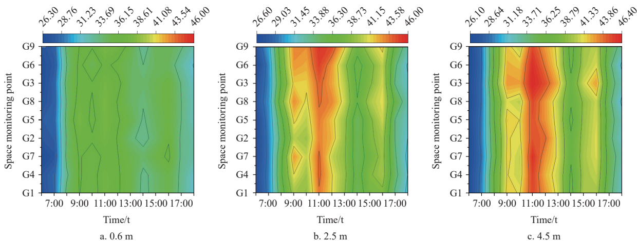
Figure 3 Contour cloud map of different monitoring plane temperatures in the greenhouse
