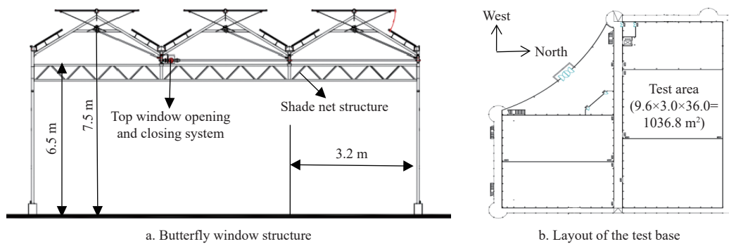
Figure 1 Schematic diagram of the layout and structure of the experimental greenhouse
