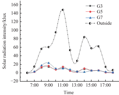
Figure 8 Changes in the average solar radiation intensity at different monitoring heights in the greenhouse at each moment
