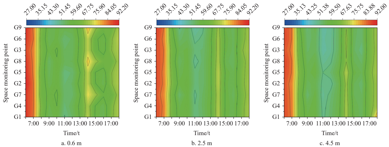
Figure 5 Humidity changes at different monitoring heights in the greenhouse
