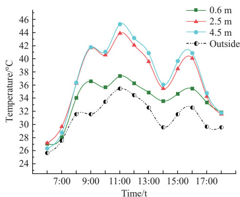
Figure 4 Average temperature and outdoor temperature changes at different monitoring heights in the greenhouse at each time
