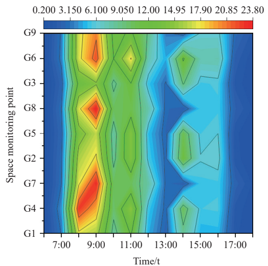
Figure 7 Contour cloud map of solar radiation intensity at 1.5 m in the greenhouse
