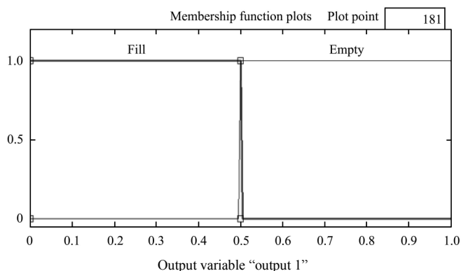
Figure 8 Membership Function (MF) for output ("Output1")
