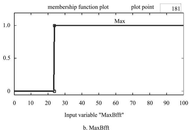
Figure 7 Membership Function (MF) for Average and MaxBfft
