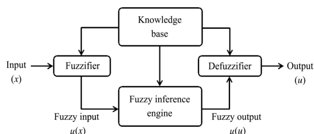
Figure 4 Block diagram of Mamdani fuzzy inference system
