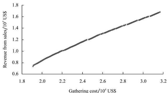
Figure 1 Efficient frontier with 282 solutions to the objectives of maximization of revenue from electricity sales and minimization of gathering cost
