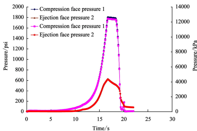
Figure 4 Typical pressure exerted on hay by the main compression and ejector rams over the duration of a test. Pressure 1 was measured by pressure transducer 1 in the compression face; Pressure 2 was measured by pressure transducer 2 in the ejection face
