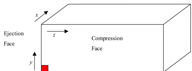
a. Typical compressed bale dimensions ( x = 0.432 m; y = 0.432 m; z = 1.168 m)
