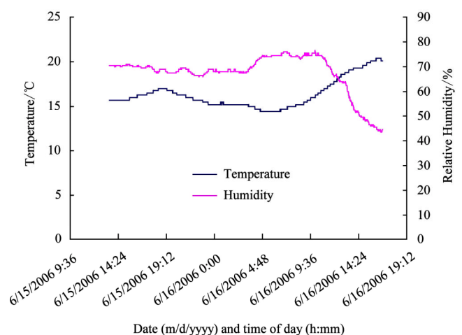
Figure 3 Temperature and relative humidity during the field test
