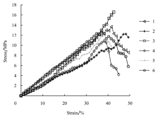
Figure 9 Reed sheared stress-strain curve
