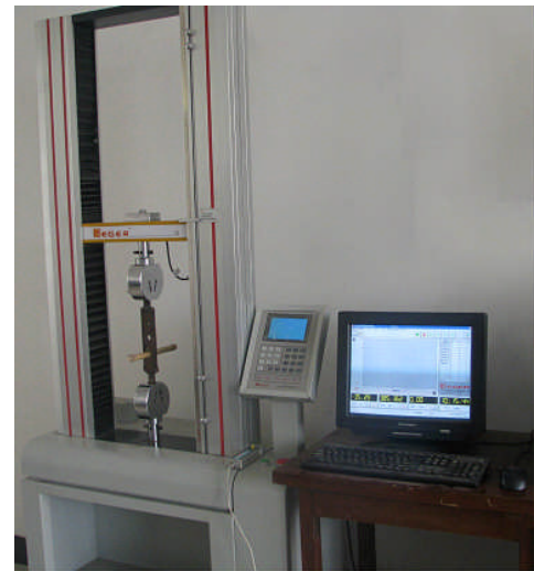
Figure 2 Structural diagram of the measurement system
