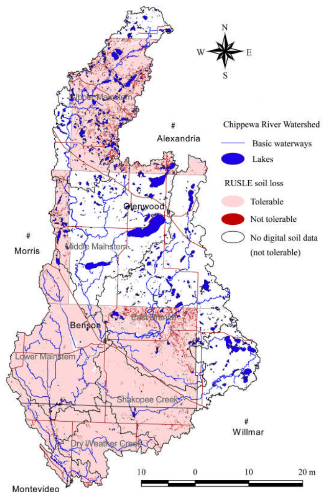
Figure 4 RUSLE results
