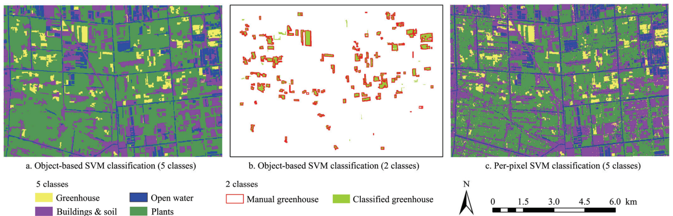
Figure 3 Maps of classification results obtained via object-based classification and per-pixel classification based on the SVM approach
