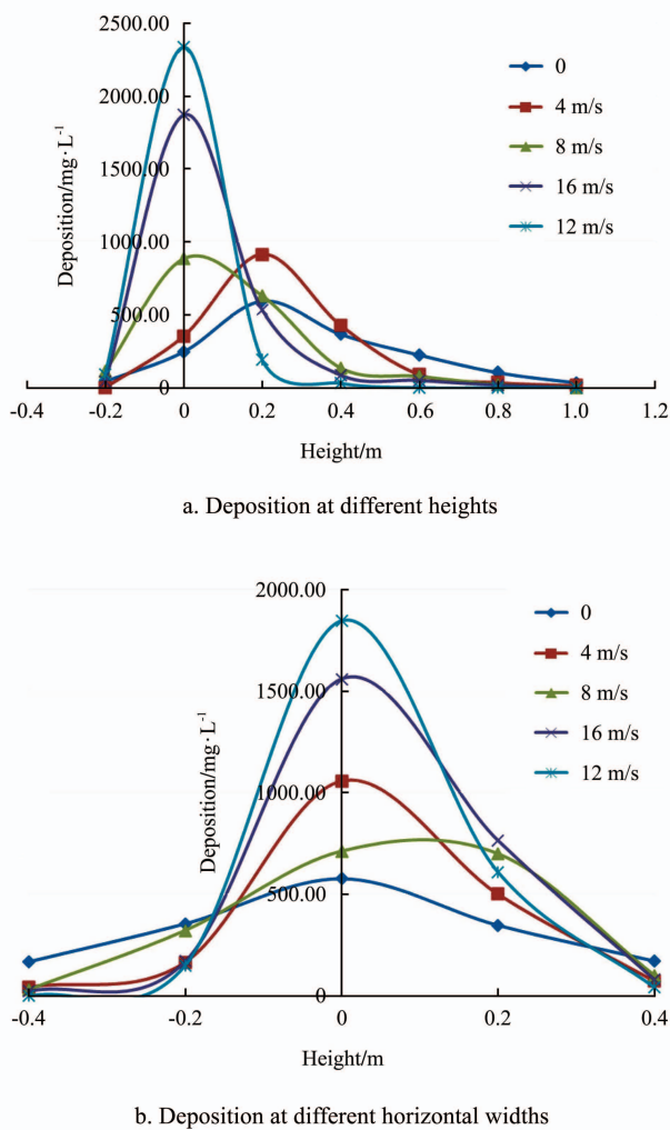
Figure 8 Effects of wind speed on droplet deposition at different positions
