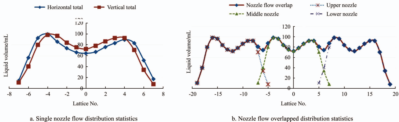
Figure 7 Statistical results of nozzle flow distribution
